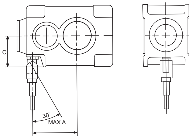
TYPE B2S
