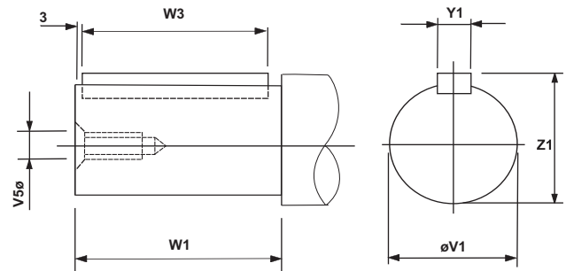
Output Shaft
