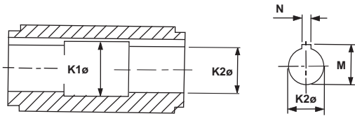
Sizes 160 & 140 only
