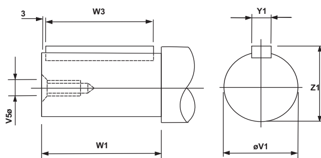
Output Shaft
