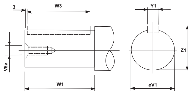
Output Shaft
