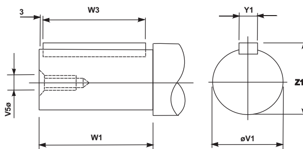
Output Shaft
