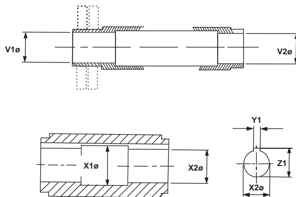
Output Sleeve Bores
