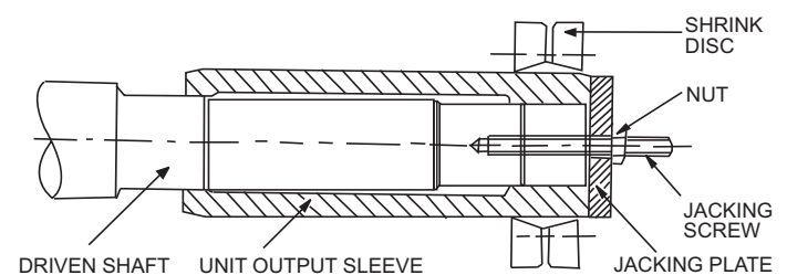
FIG.3 MOUNTING GEAR UNIT
